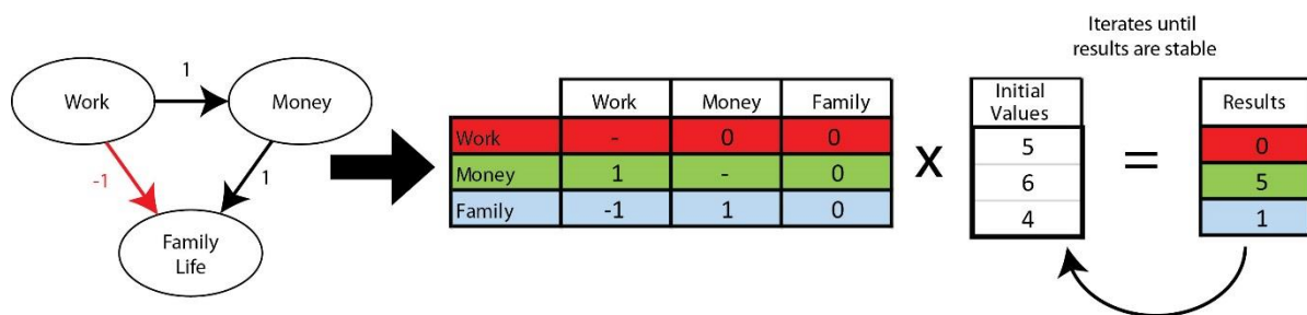
Figure 13: Schematic diagram of simulation using Fuzzy Cognitive Mapping.
